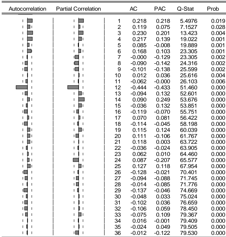
Fig 5: ACF and PACF Plot of \Delta^{12}\text{dlog}(\text{ER}_t)
