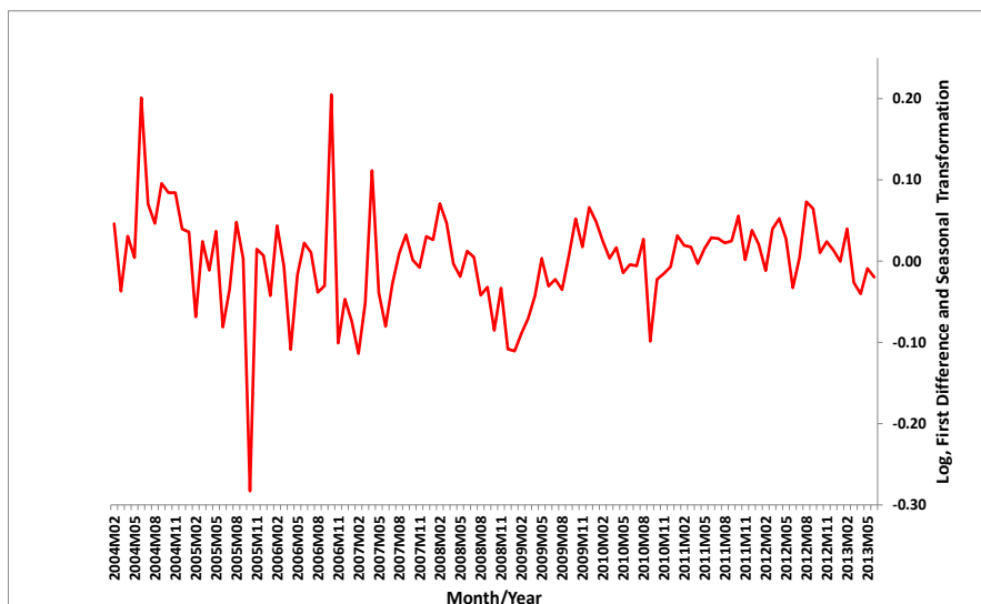
Fig 4: Time Plot of Transformed External Reserves Data ( \Delta^{12}\text{dlog}(\text{ER}_t) )
