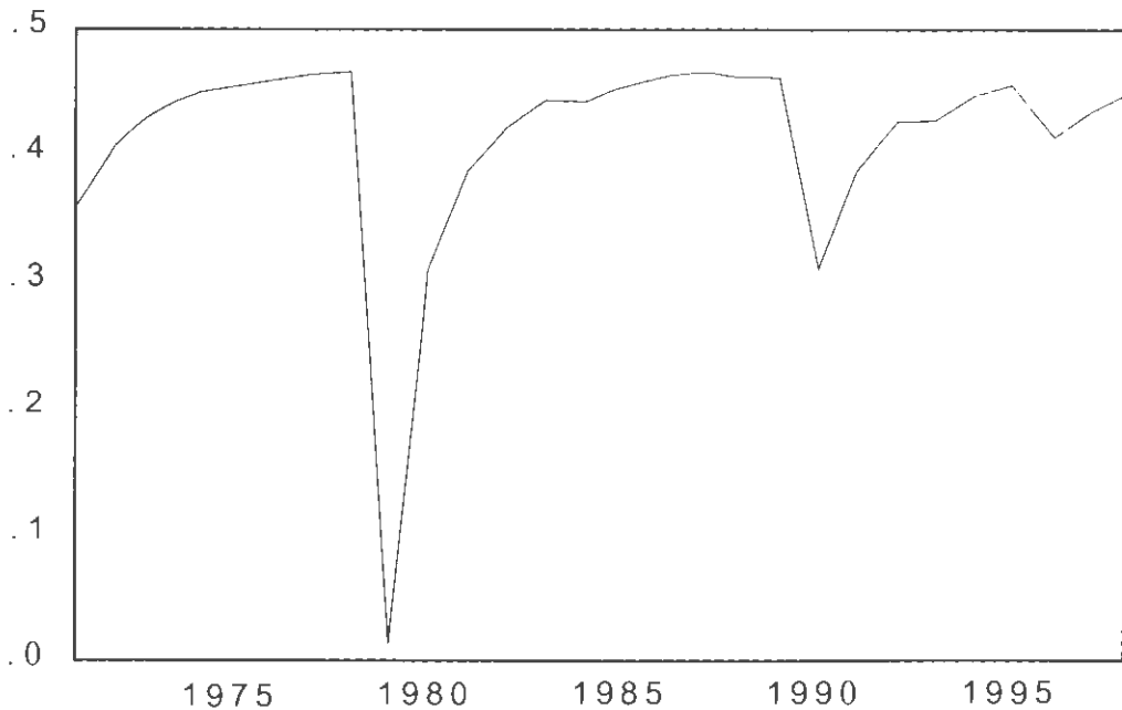
Graph of the Generalised Autoregressive Condition Heteroscedasticity (GACH) Model
